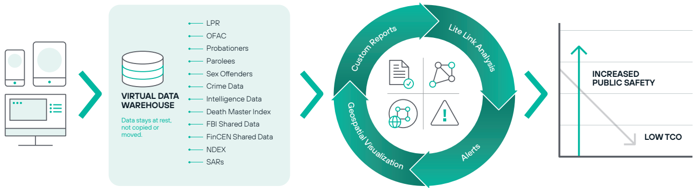
Figure 1: Federated searching across the enterprise coupled with automated discovery tools and lite-analytics supports intelligence-led investigations
